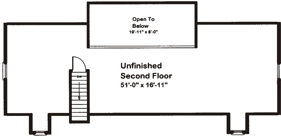
Optional Second Floor Plan (910 Sq Ft)
